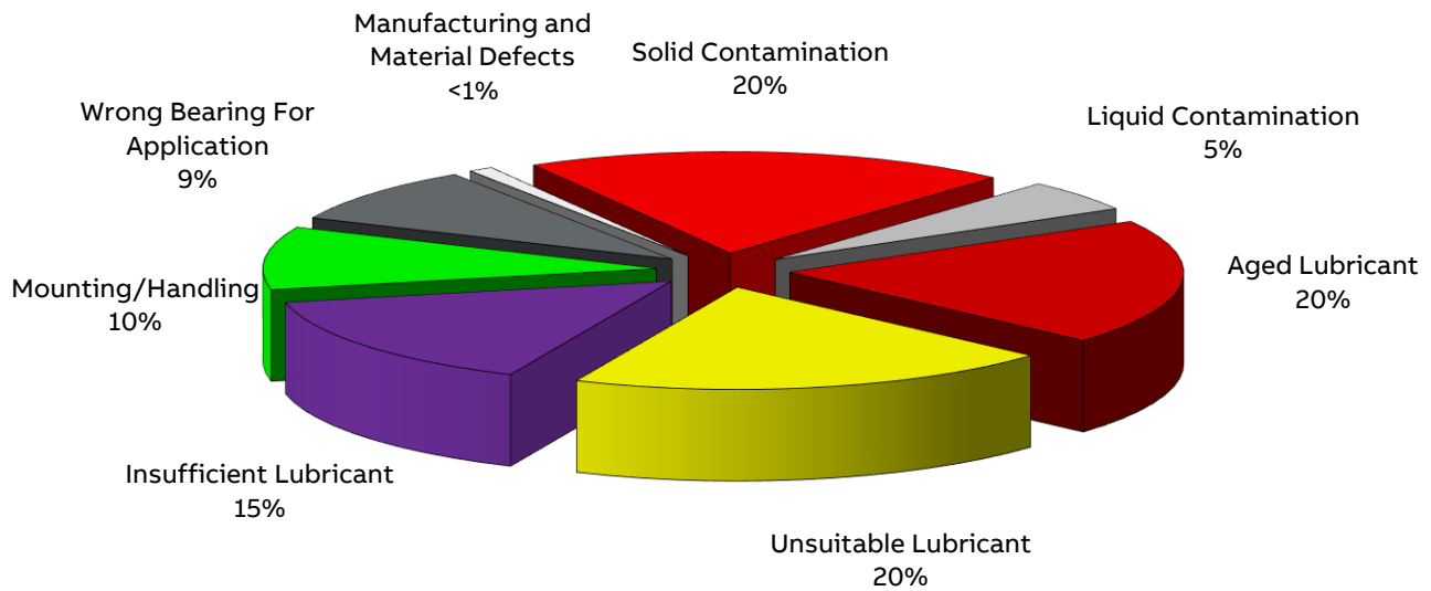
Figure 1. Industry Percentage of Bearing Failure Modes [5] [6]
