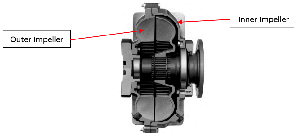
Figure 1. Fluid coupling section view
