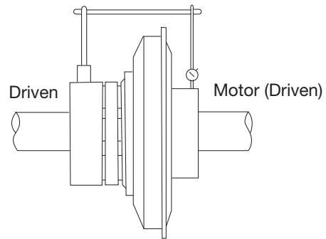
Figure 2 - Parallel Misalignment
