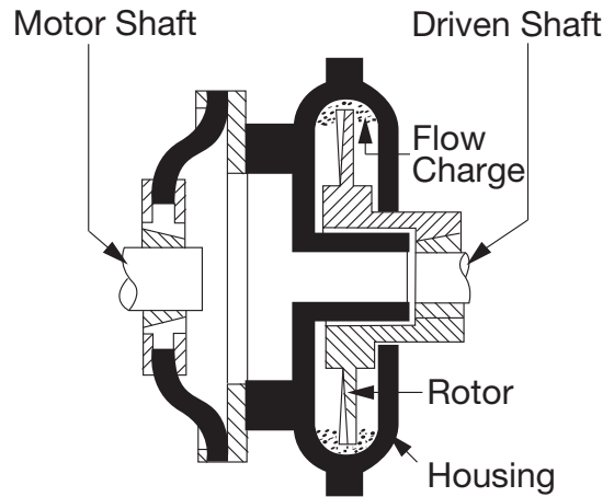
Figure 1 - Housing Cross Section
