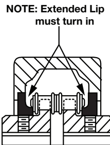
Figure 3 - "L" Shaped Rubber Ring
