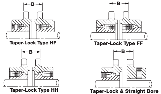
Figure 1 - "B" Dimension
