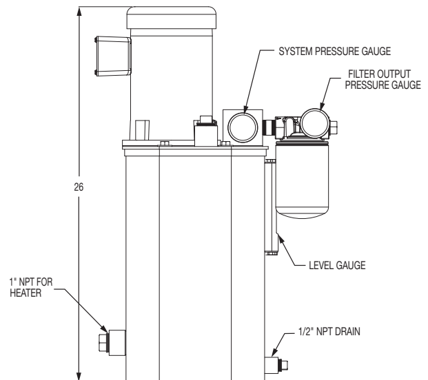
Figure 2 - OLF-2 Dimensions
