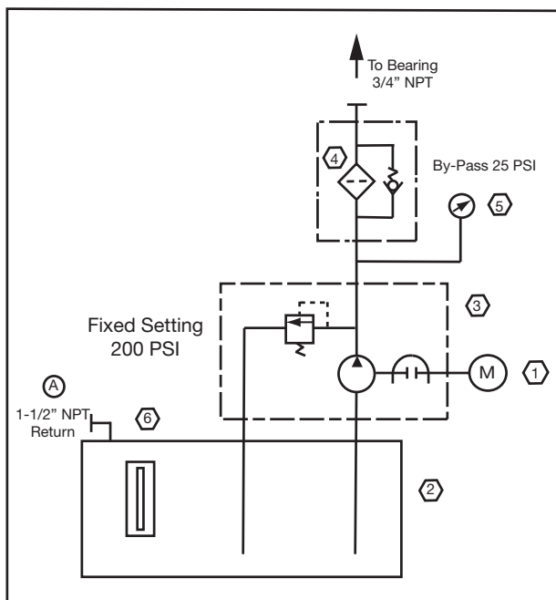
Figure 1 - Wiring Diagram
