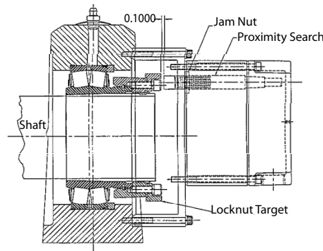
Figure 7: ISAF Housing with Speed Kit
