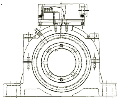
Figure 6: ISAF Housing with Thermocouple
