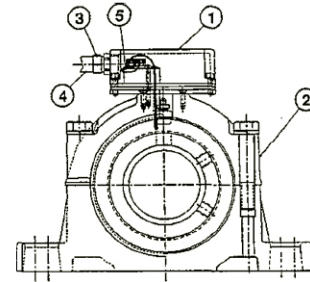
Figure 3: TAF Housing with Thermocouple
