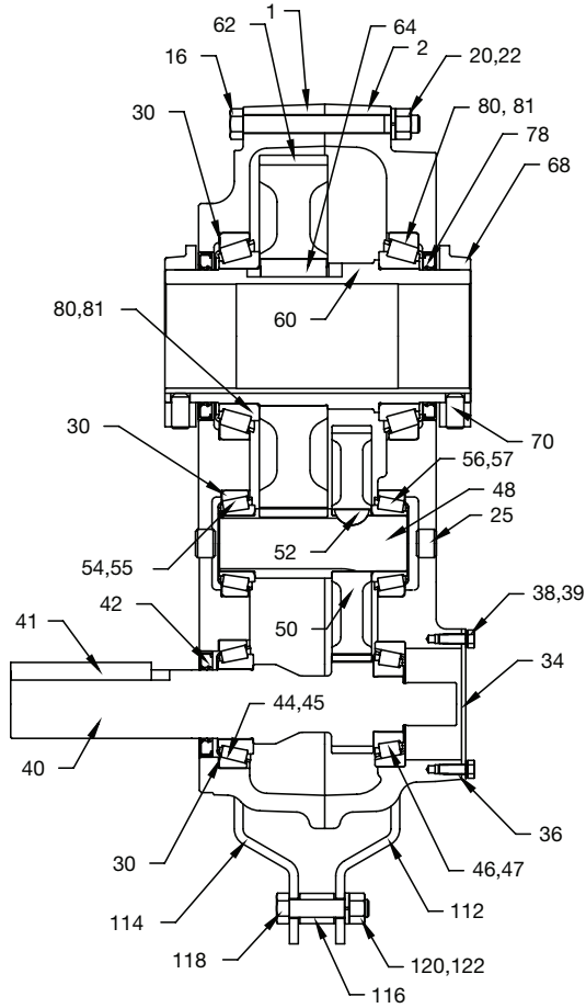
STRAIGHT BORE
