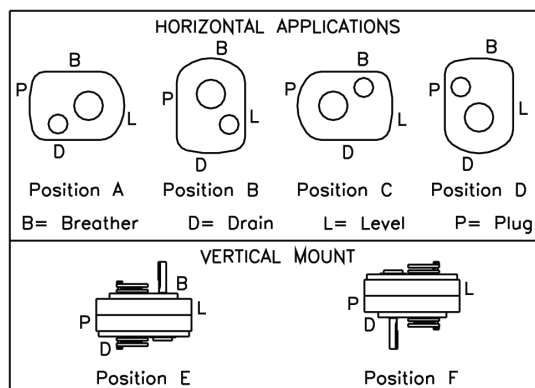
Figure 1 - Mounting Positions
