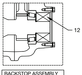
BACKSTOP ASSEMBLY
