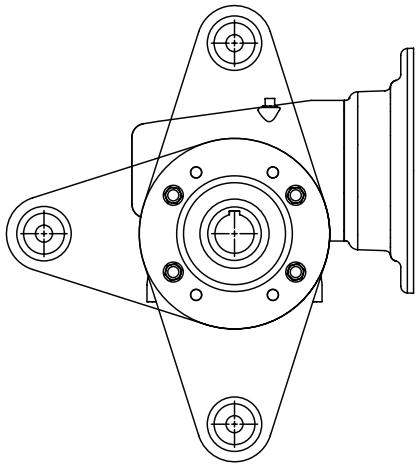
Figure 2 - Stainless Steel Torque-Arm Possible Mounting Positions
