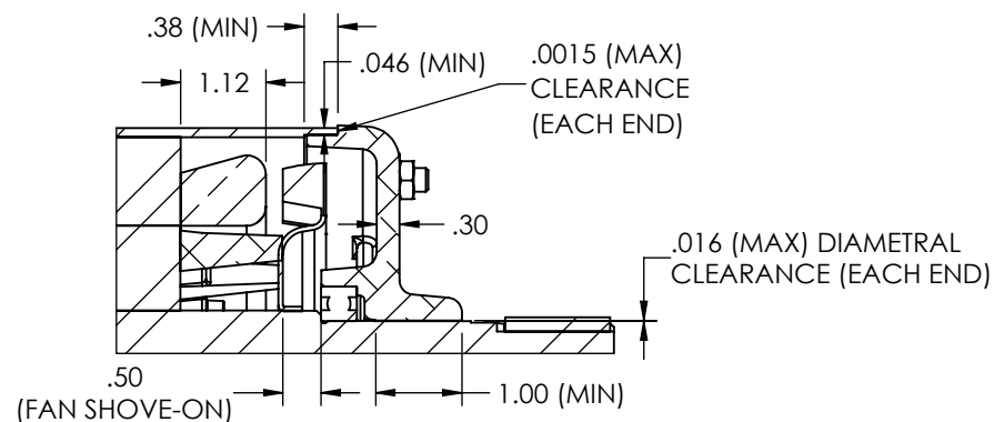
PULLEY END DETAIL
