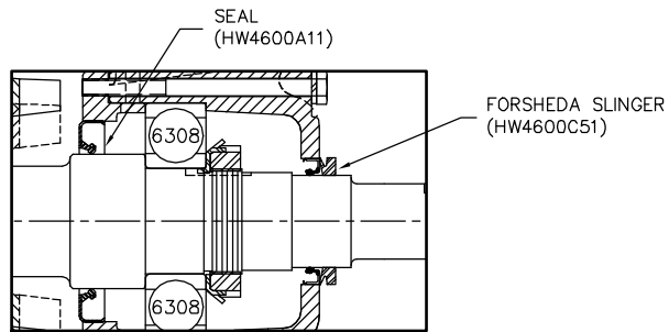
PULLEY DETAIL
