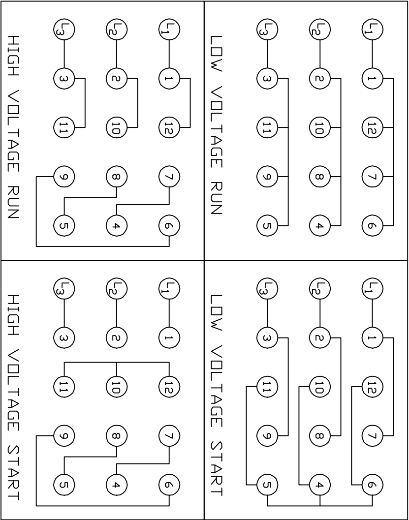
DUAL VOLTAGE Y START \Delta RUN
