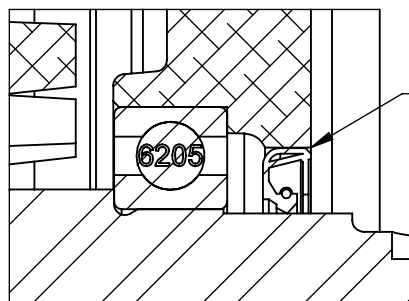
PULLEY END DETAIL
