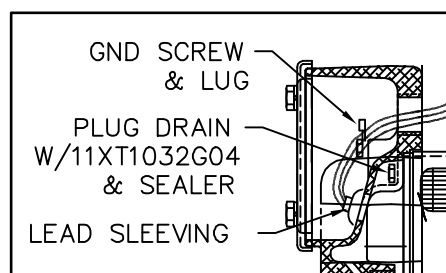
FRONT END DETAIL
