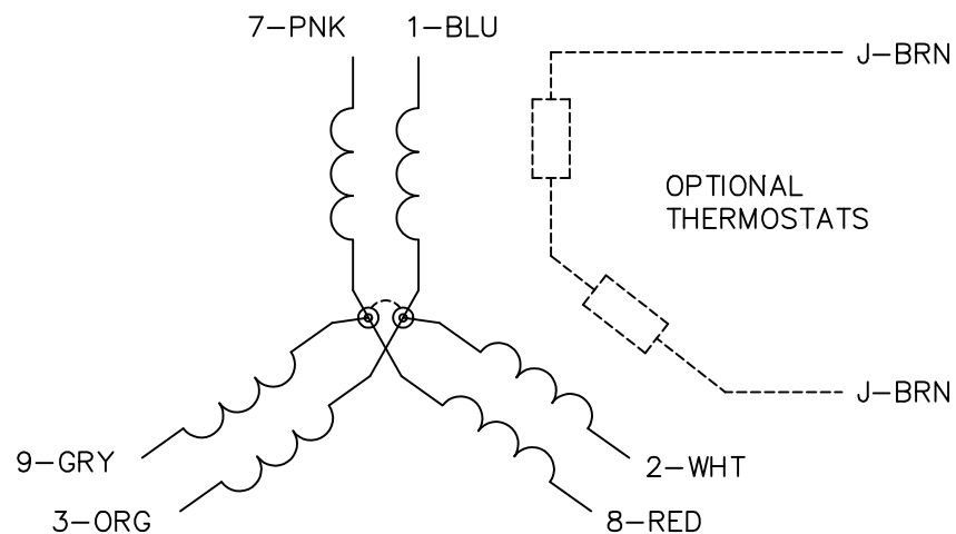
TYPICAL WYE-CONNECTED MOTOR
