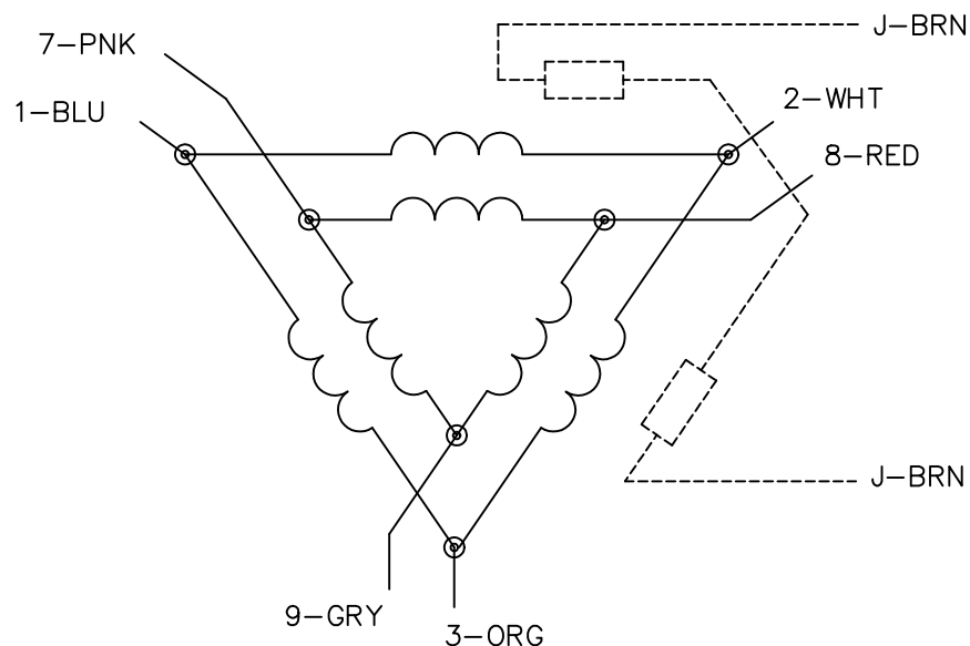
TYPICAL DELTA-CONNECTED MOTOR
