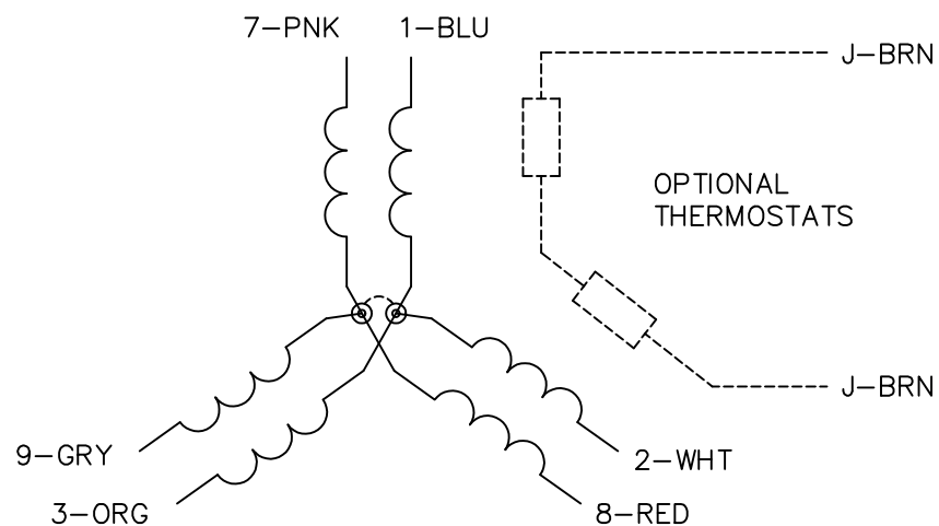
TYPICAL WYE-CONNECTED MOTOR
