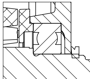
DRIVE END DETAIL
