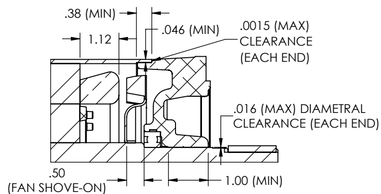
PULLEY END DETAIL
