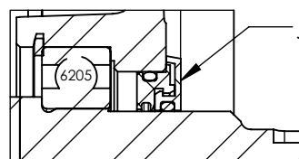
PULLEY END DETAIL
