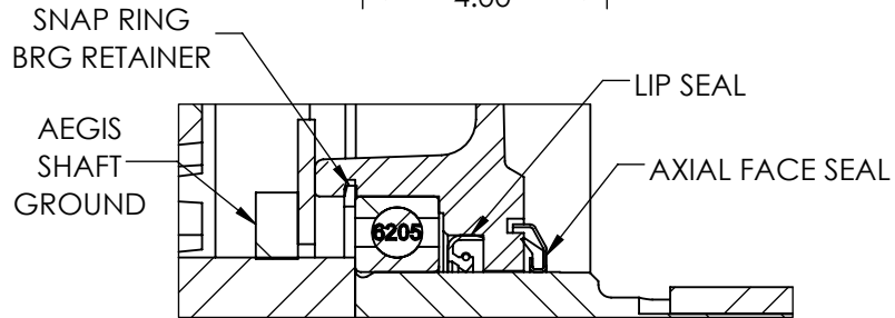
PULLEY END DETAIL
