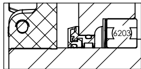
FRONT END DETAIL
