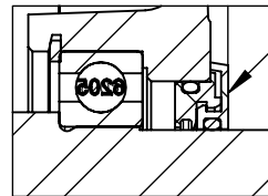
PULLEY END DETAIL
