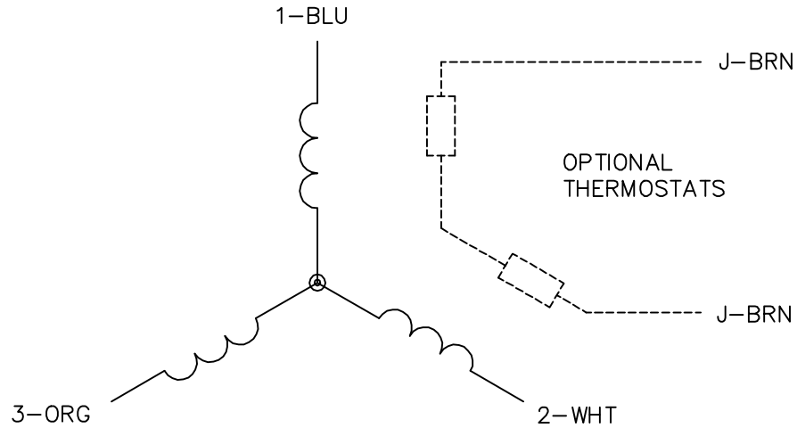
TYPICAL WYE-CONNECTED MOTOR
