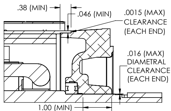
PULLEY END DETAIL
