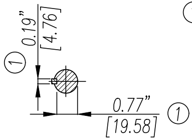
Keyseat detail Detalle Cuñero
