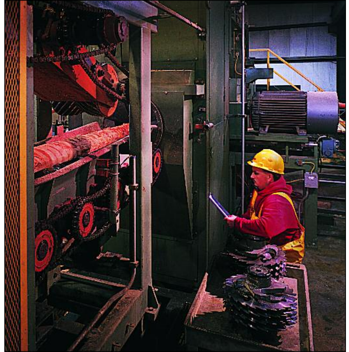
A Baldor 500 hp, medium voltage Chemical Processing Motor (pictured at the back end of the machine) and Series 22H Line Regen Vector Control run this chipping machine at a North Carolina lumber mill. High performance and reliability are the hallmarks of this Baldor motor, running in multiple shifts, under high-torque demands, exposed to sawdust and other airborne contaminants.
