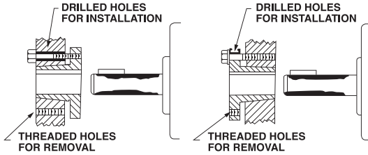
Figure 1 - Conventional Mounting
