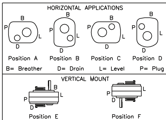
Figure 1 - Mounting Positions
