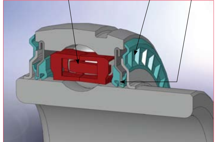
Maxlife Cage Rubberized Flinger Triple Lip Seal
